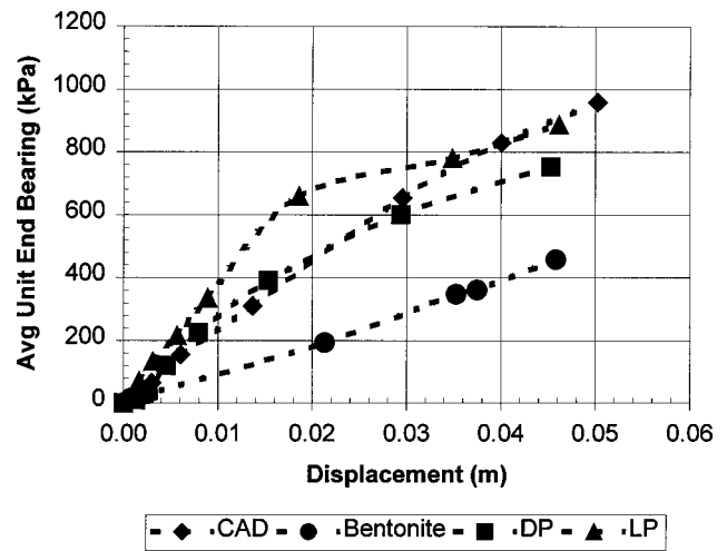
Fig. 7. Load transfer in end bearing
