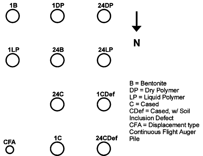
Fig. 1. Test site layout (no scale)
