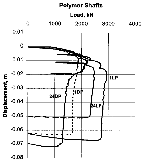
Fig. 2. Load-deflection response of polymer shafts
