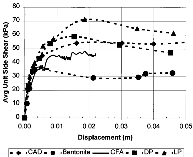
Fig. 6. Load transfer in side shear
