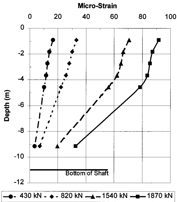
Fig. 5. Strain distribution, shaft 1 DP
