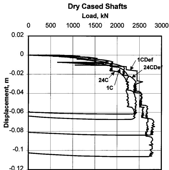
Fig. 4. Load versus deflection response of dry cased shafts
