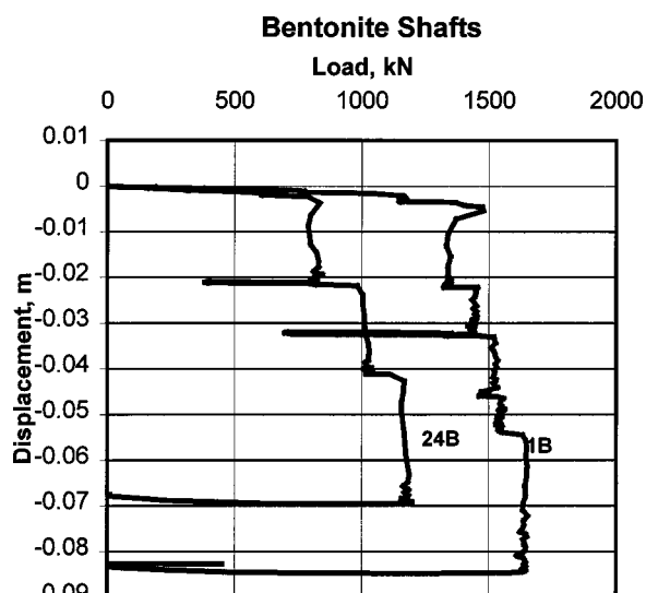
Fig. 3. Load versus deflection response of bentonite shafts
